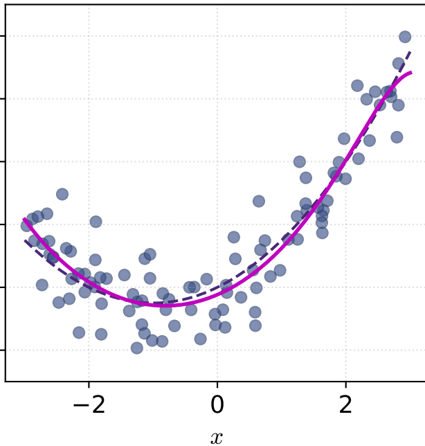
Ridge (alpha=1)
